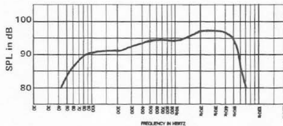
FIGURE 2 - TL606/EVM .15L Frequency Response (Swept 1/3-Octave Band Pink Noise, 4 V at 10 ft. on Axis, Half-Space Environment)
